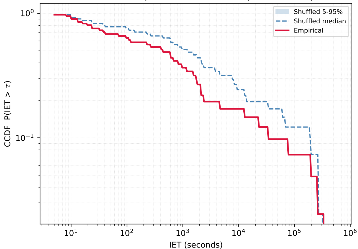
User 261376227 - Empirical vs Reshuffled | KS=0.200 p=0.000
